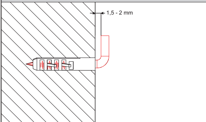
Detail 3.2
